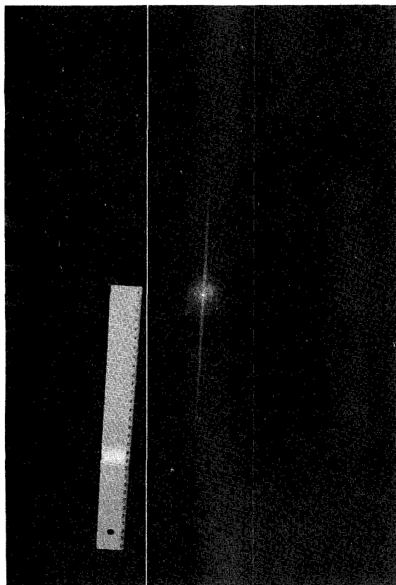
Figure 5. The diffraction pattern obtained on a white screen by illuminating a horizontal razor blade with a laser beam.
