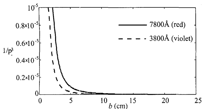
Figure 4. Values of 1/p^3 for different values of b .
