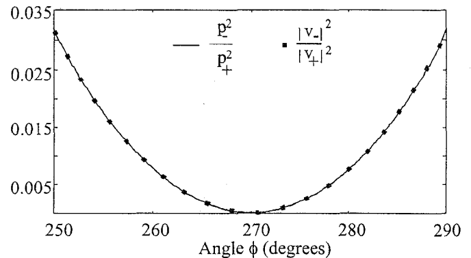
Figure 9. The ratio between of the magnitudes of the two terms 1/p_+^2 and 1/p_-^2 (solid line), and of the magnitude of the terms |v_+|^2 and |v_-|^2 (dots).
