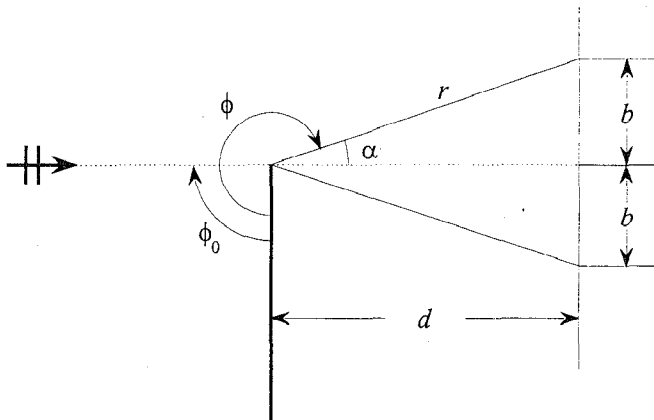
Figure 3. The geometry of the half-plane scattering problem.
