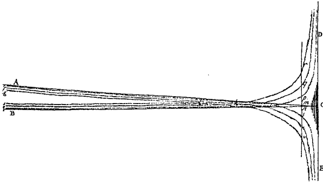
Figure 7. Newton's drawing of interference fringes in Obs. 10.
