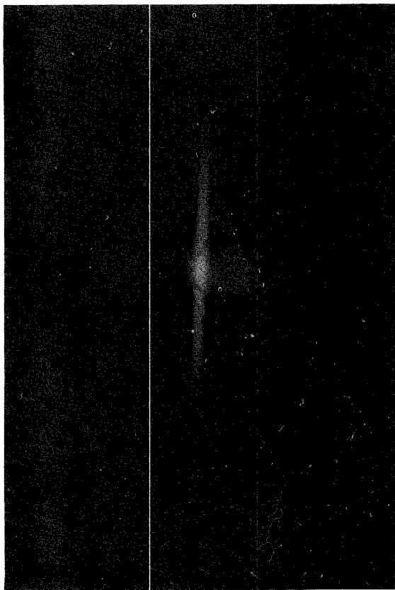
Figure 10a. Laser ray diffraction fringes, \lambda = 6328\text{\AA} .
