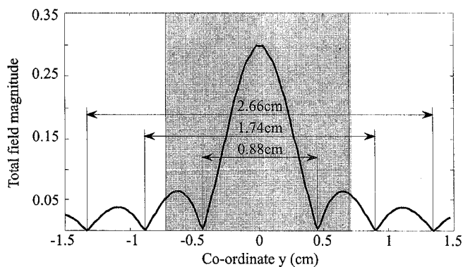
Figure 12. The field nulls along the line rv . The shadowed region corresponds to the Fresnel region; the regions to the right and the left are ray regions ( \lambda = 6328 \text{ \AA} ).
