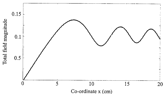
Figure 14. Field minima along the x axis ( \lambda = 6328 \text{ \AA} ).
