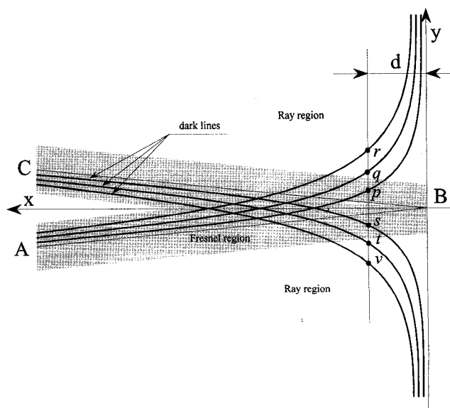
Figure 11. A schematic diagram of the interference fringes. On this duplicate of Newton's Figure (Figure 7 of the present paper), the Fresnel region is shadowed. It is evident how the hyperbola branches near the vertical asymptote are in the ray region.
