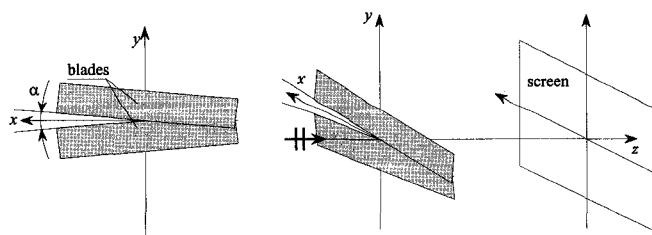
Figure 6. The configuration of Obs. 8 and 10.
