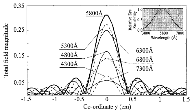
Figure 13. The field magnitude along a line rv at different frequencies. The fields are weighted by the human eye's response curve, shown at the top right.
