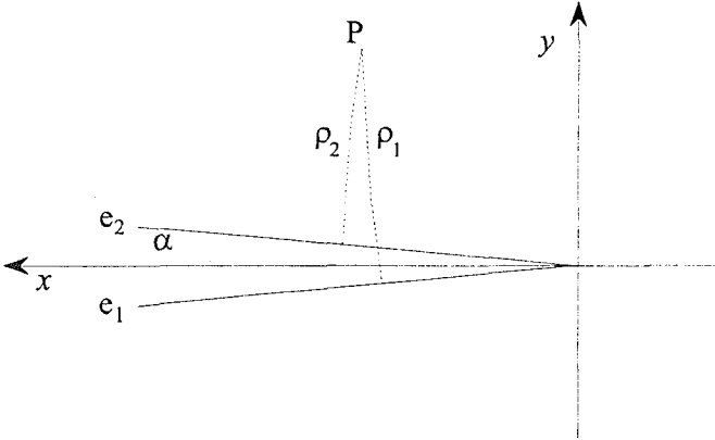
Figure 8. The projection of the diffracted rays onto a z = \text{const} plane.
