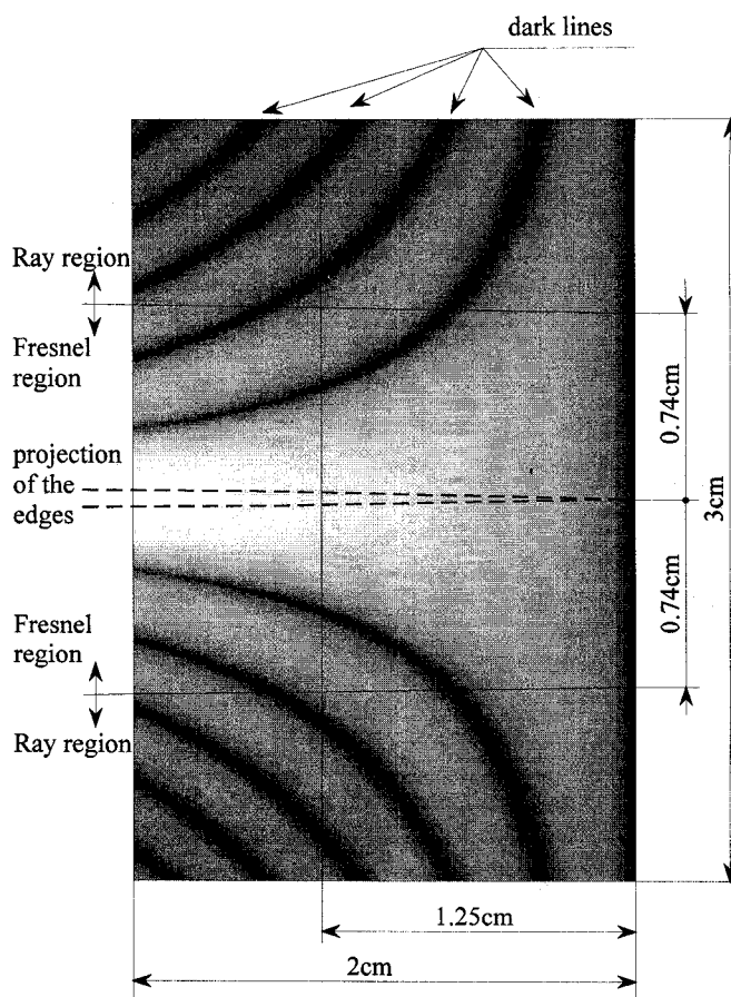
Figure 10b. A numerical field evaluation of the diffraction fringes ( \lambda = 6328\text{\AA} ). To better show the interference fringes, the field map shows the logarithm of the field magnitude. The limits of the ray region are also indicated.
